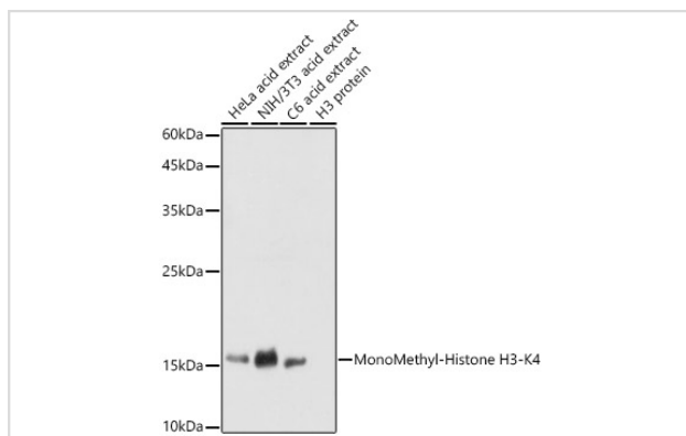
Western blot analysis of extracts of various cell lines, using MonoMethyl-Histone H3-K4 antibody.
