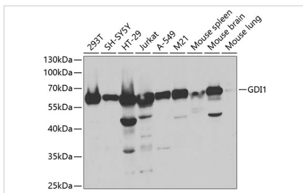
Western blot analysis of extracts of various cell lines, using GDI1 antibody.
