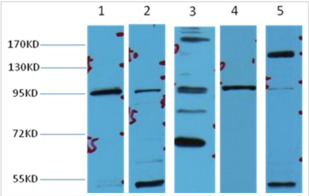
Western blot analysis of 1) Hela, 2) 293T, 3) MCF7, 4) Mouse Brain tissue ,3) Rat LiverTissue, using #38020 diluted at 1:2,000
