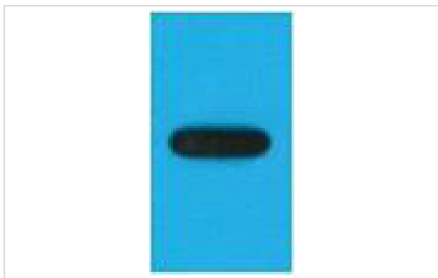
Western blot analysis of recombinant EYFP protein, diluted at 1:10000.
