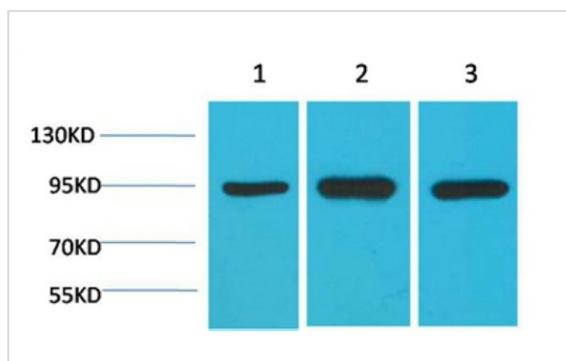
Western blot analysis of 1) Hela, 2) Mouse Brain Tissue, 3) Rat Brain Tissue with HSP90 \alpha Mouse mAb diluted at 1:2,000.
