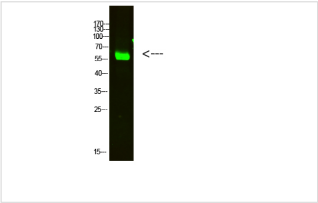
Western Blot analysis of HELA cells using primary antibody diluted at 1:2000(°C overnight). Secondary antibodyB£B1Goat Anti-rabbit IgG IRDye 800( diluted at 1:5000, 25B'Γ£C, 1 hour)
