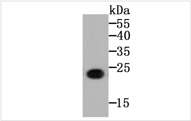
Western blot analysis of CD130 on CD130 recombinant protein using anti-CD130 antibody at 1/5,000 dilution.
