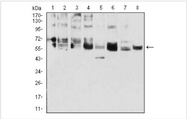
Western blot analysis of CK5 on different cells lysates using anti-CK5 antibody at 1/1,000 dilution. Positive control \Omega\frac{1}{2}\Omega\frac{1}{2} Line1: A431 Line2: 3T3-L1 Line3: COS7 Line4: MCF-7 Line5: SK-Br-3 Line6: Hela Line7: Lncap Line8: HepG2
