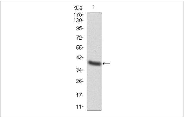
Western blot analysis of AP2 alpha on human AP2 alpha recombinant protein using anti- AP2 alpha antibody at 1/1,000 dilution.
