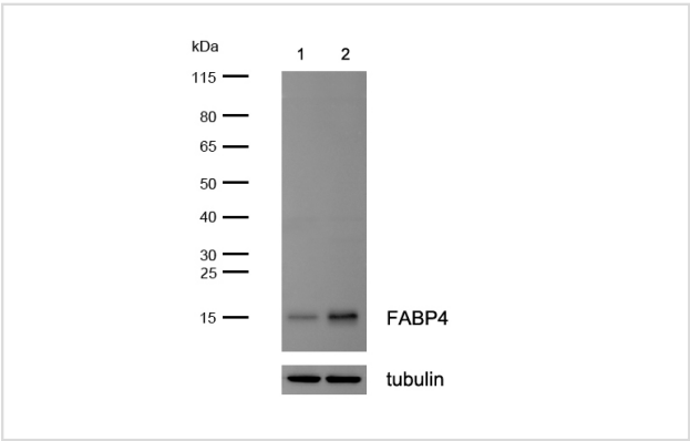
All lanes : FABP4 Rabbit mAb at 1/1k dilution Lane 1 : FABP4 knockout HAP1 cell lysate Lane 2 : Wild-type HAP1 cell lysate Lysates/proteins at 20 µg per lane.
