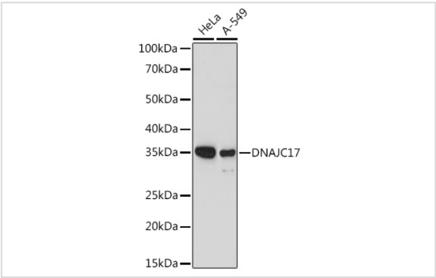
Western blot analysis of extracts of various cell lines, using DNAJC17 antibody.
