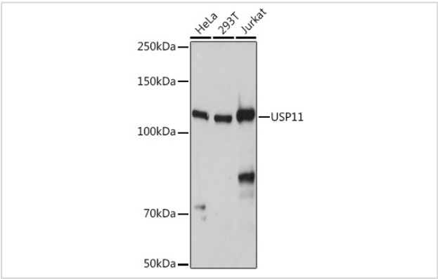
Western blot analysis of extracts of various cell lines, using USP11 antibody.
