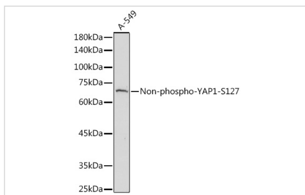
Western blot analysis of extracts of A-549 cells, using Non-phospho-YAP1-S127 antibody.
