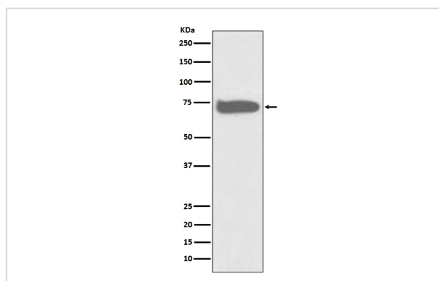
Western blot analysis of GCLC expression in HepG2 cell lysate.
