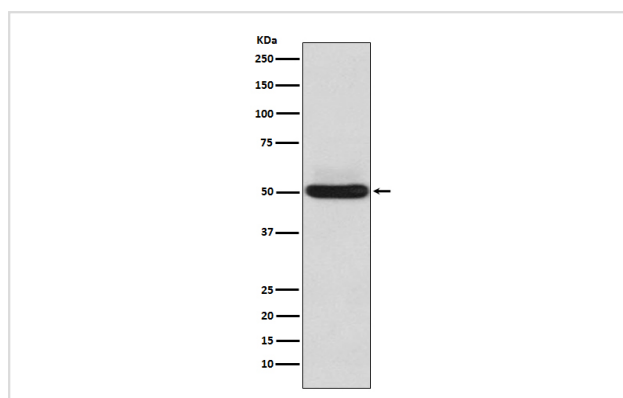
Western blot analysis of alpha Sarcoglycan expression in Human skeletal muscle lysate.
