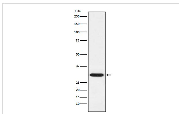
Western blot analysis of GCLM expression in K562 cell lysate.
