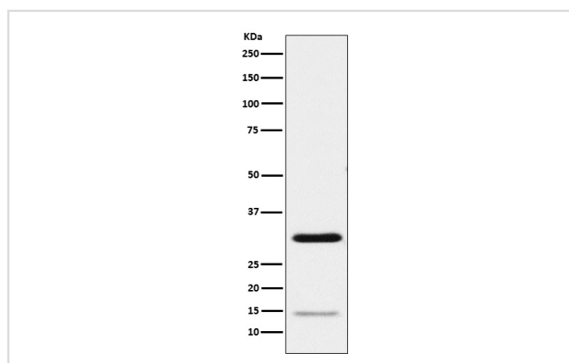
Western blot analysis of Geminin expression in HeLa cell lysate.
