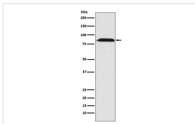
Western blot analysis of Furin expression in HepG2 cell lysate.
