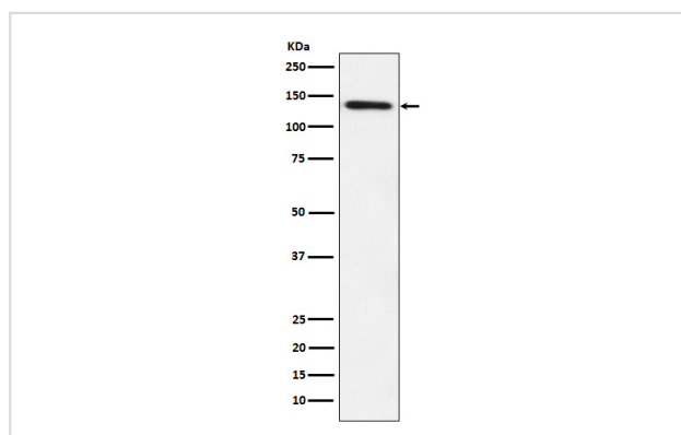
Western blot analysis of Lipin 1 expression in HepG2 cell lysate.
