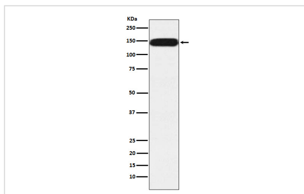
Western blot analysis of Pumilio 1 expression in HeLa cell lysate.
