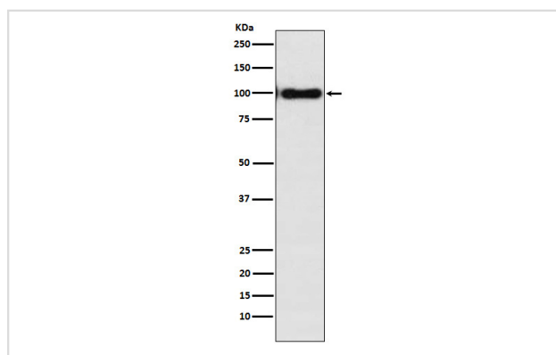
Western blot analysis of Desmocollin?3 expression in A431 cell lysate.
