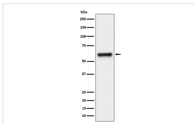
Western blot analysis of FPGS expression in HeLa cell lysate.
