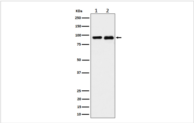
Western blot analysis of CSDE1 expression in (1) K562 cell lysate; (2) PC-12 cell lysate.
