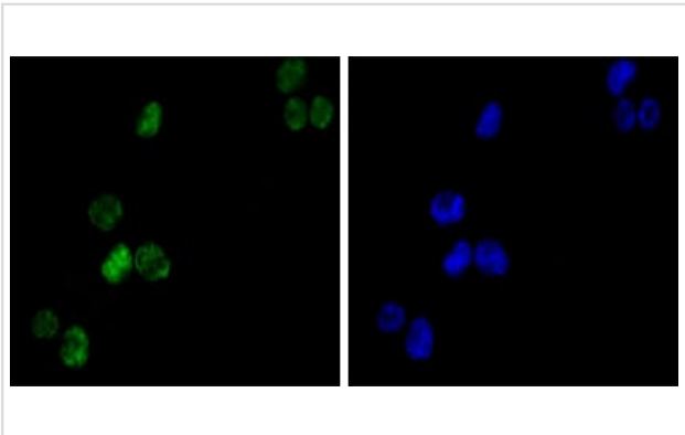
Immunofluorescence analysis of K562(left) cells using GATA1 mouse mAb (green). Blue: DRAQ5 fluorescent DNA dye.
