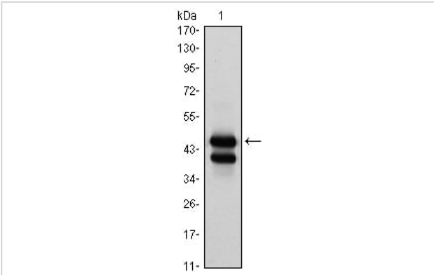
Western blot analysis using GATA1 mouse mAb against K562 (1) cell lysate.
