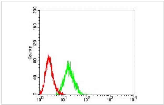
Flow cytometric analysis of HL-60 cells using KMT5A mouse mAb (green) and negative control (red).
