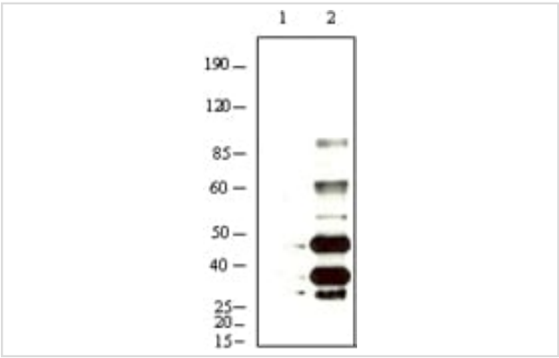
Western blot analysis using KSHV K8 mouse mAb against BCBL-1 (1) and TPA induced BCBL-1 (2) cell lysate.
