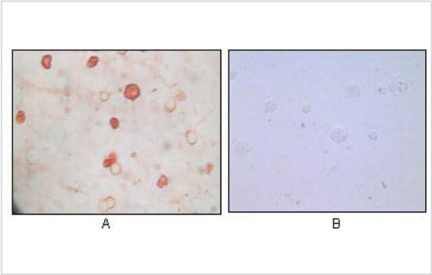
Immunocytochemistry analysis of TPA induced BCBL-1 cells (A) and uninduced BCBL-1 cells (B) using KSHV K8 mouse mAb with AEC staining.
