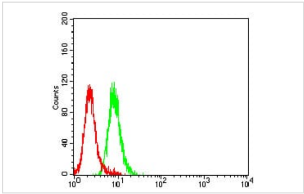
Flow cytometric analysis of Jurkat cells using ZAP70 mouse mAb (green) and negative control (red).
