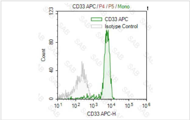
Human peripheral blood monocytes stained with APC anti-human CD33 (colored histogram) or APC mouse IgG1 (gray histogram)
