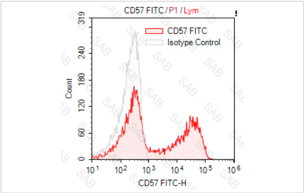
Human peripheral blood lymphocytes stained with FITC anti-human CD57 (colored histogram) or FITC mouse IgM (gray histogram)
