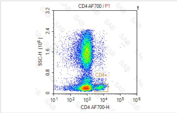
Human peripheral blood stained with Alexa Fluor 700 anti-human CD4
